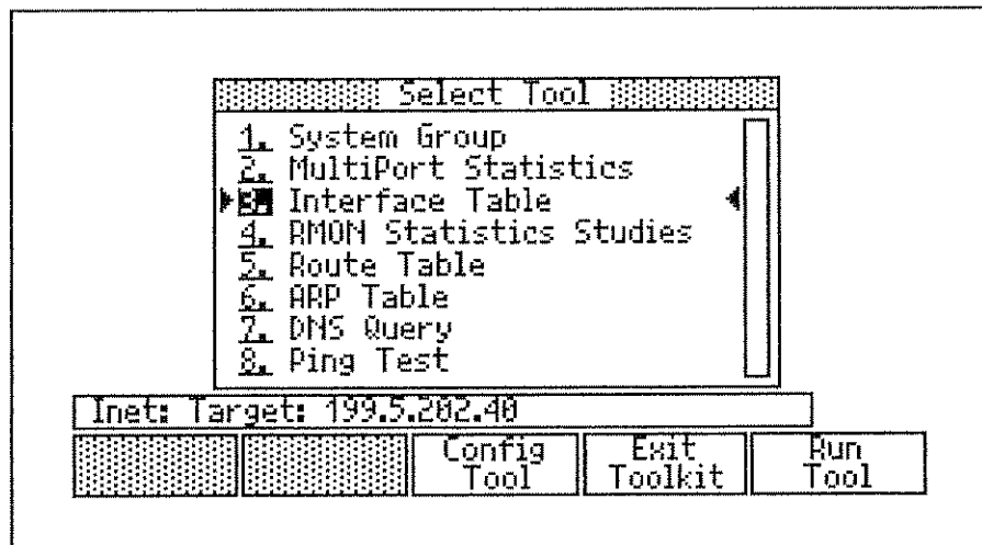
Figure 12-3. Toolkit Menu
